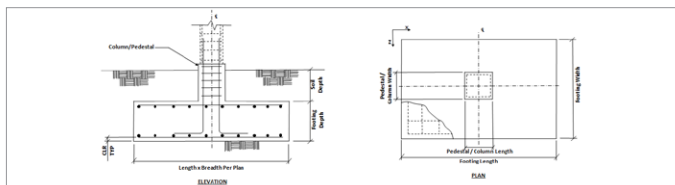
Design of isolated footings for axial load and biaxial bending with partial uplift.
