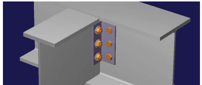
Double-angle Connection
