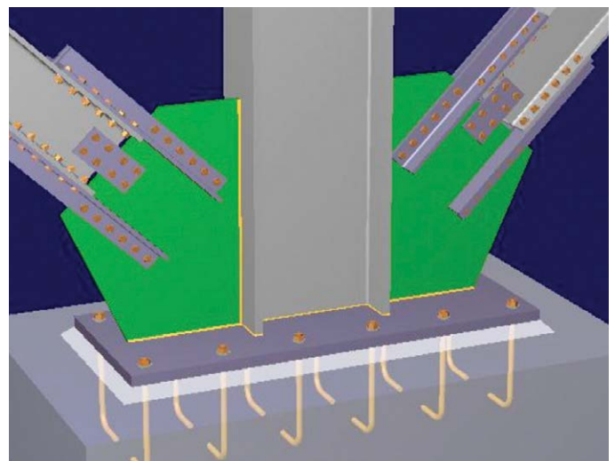
Base Plate with Gussets
