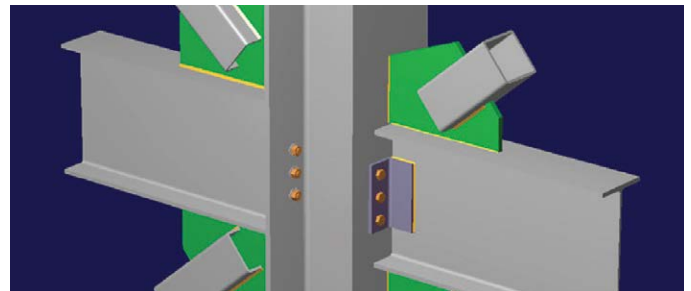
Bracing Connections
