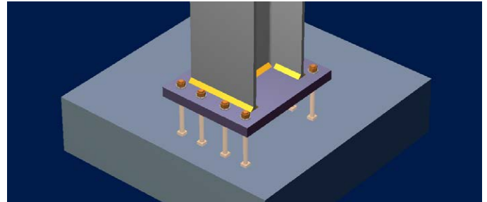
Base Plates
