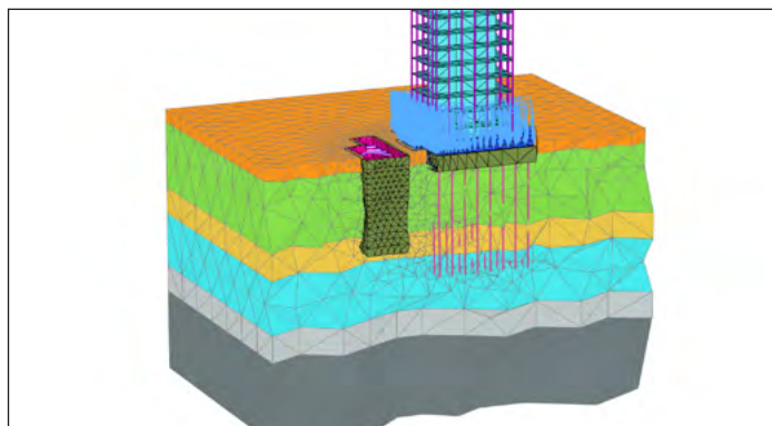
Excavation next to a building on a pile raft foundation.
