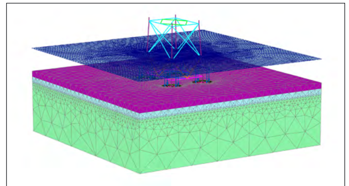
Offshore platform with suction bucket.
