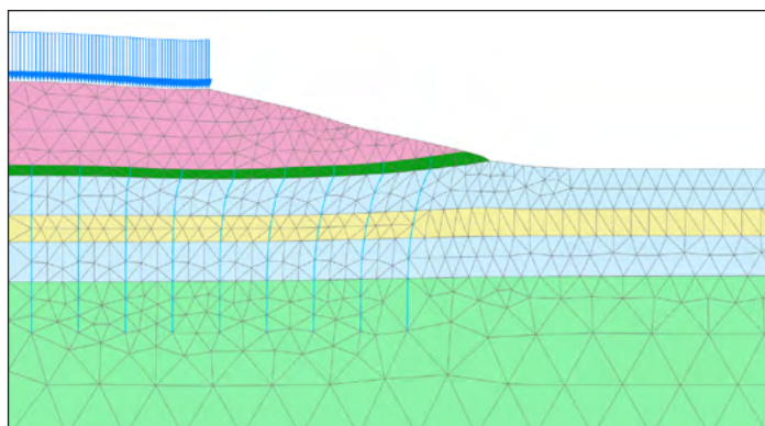
Stability of embankment on soft soil reinforced by rigid inclusions.
